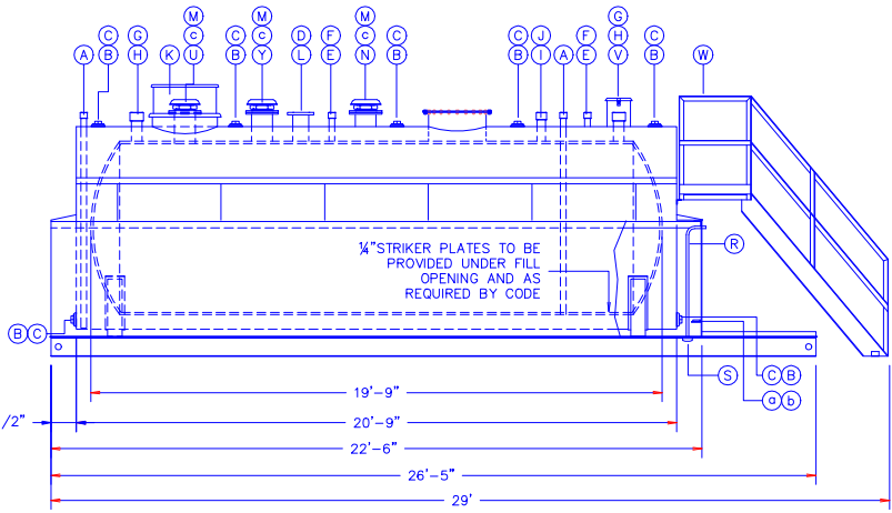
4000 GAL TANK ELEVATION SCALE: 1"=5'
