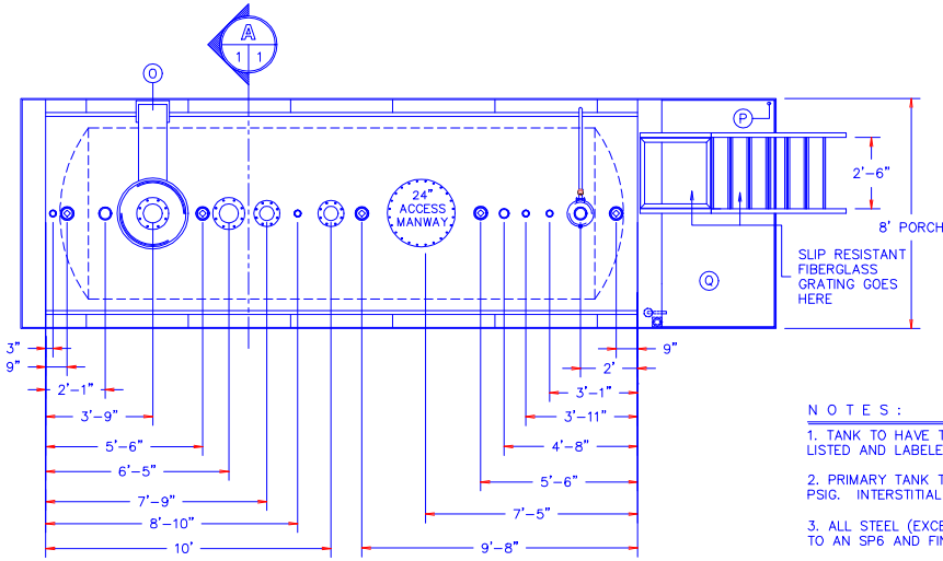
4000 GAL TANK PLAN SCALE: 1"=5'
